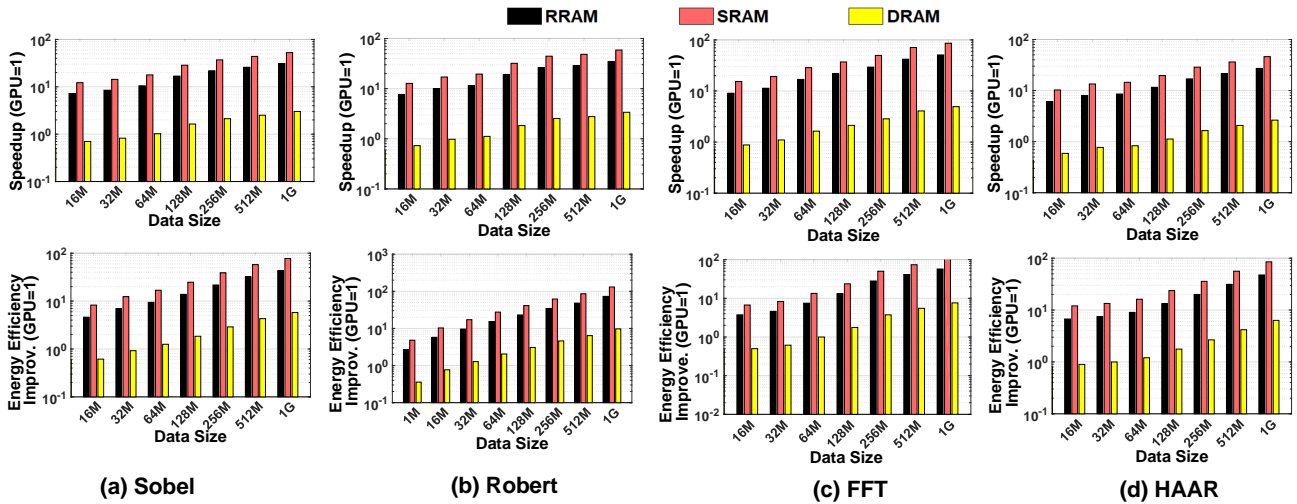
Figure 6: Speedup and energy efficiency improvement of performing PIM operation over different applications.
