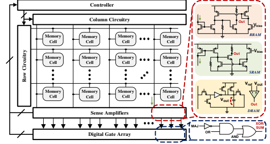
Figure 5: GPIM Overall Architecture
